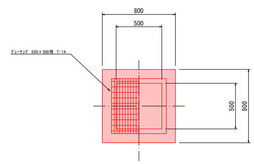
SM-B500-L500-H1050(700)
