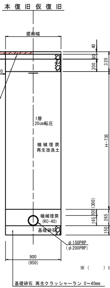
S = 1 : 30
