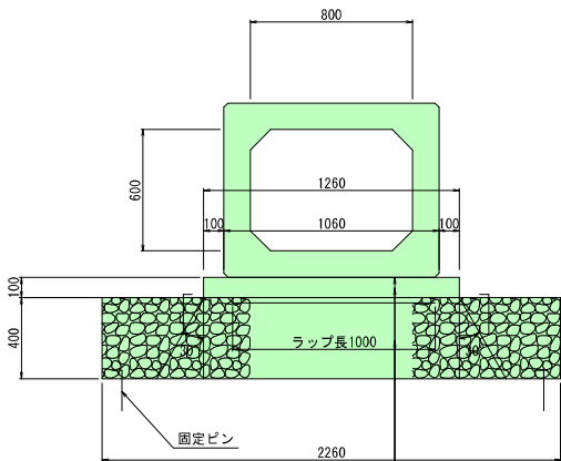
RCB-B800-H600
