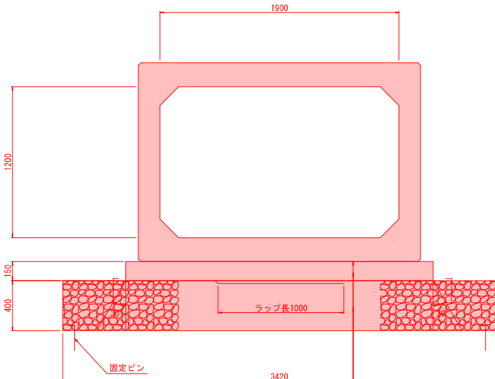
RCB-B1900-H1200
