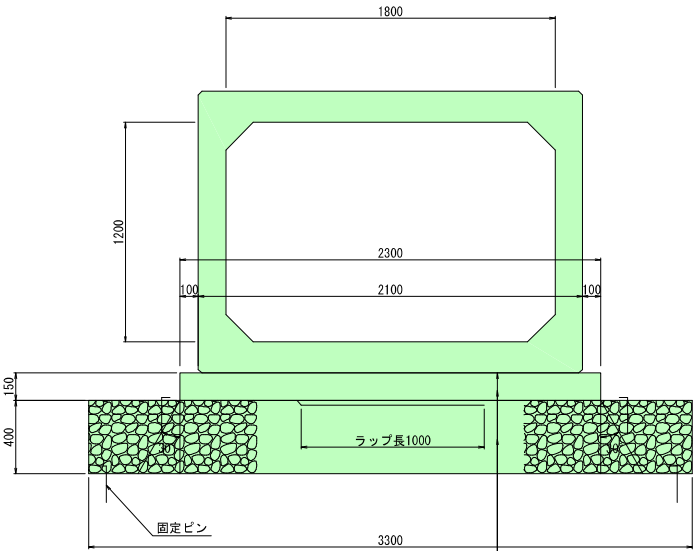
RCB-B1800-H1200
