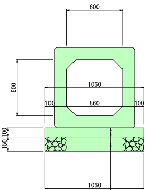
RCB-B600-H600
