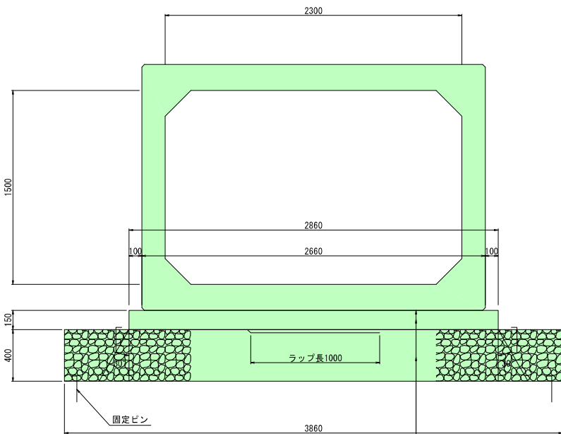
RCB-B2300-H1500
