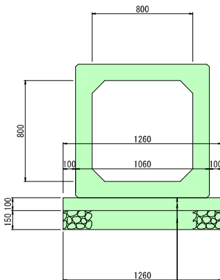
RCB-B800-H800
