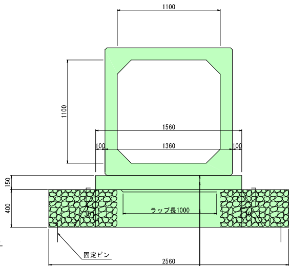
RCB-B1100-H1100
